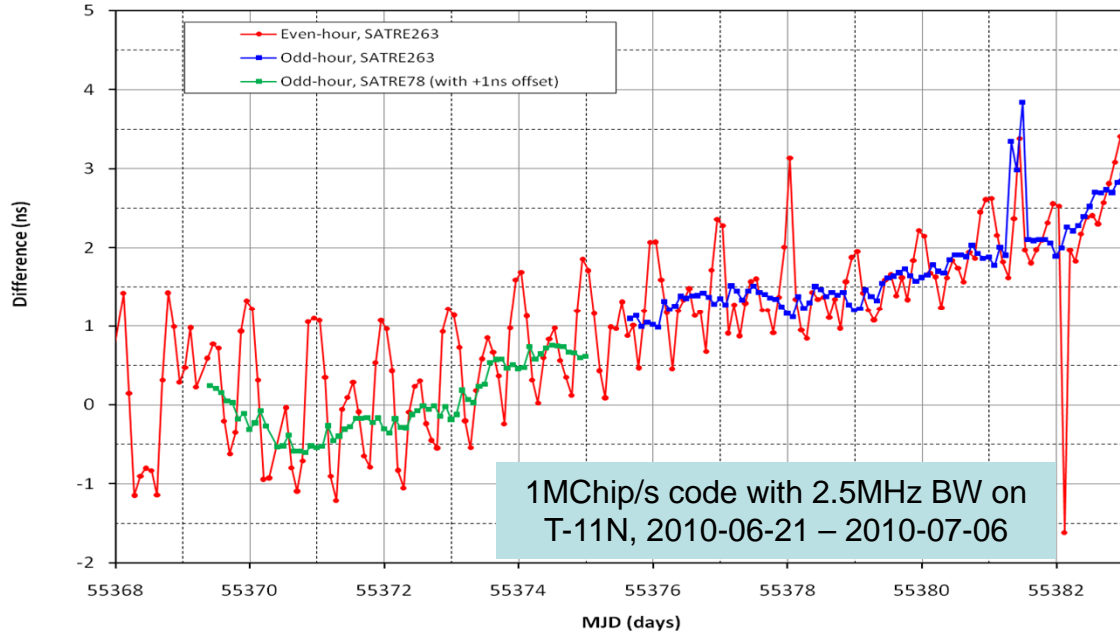
UTC(NIST)- UTC(PTB) TWSTFT Difference
