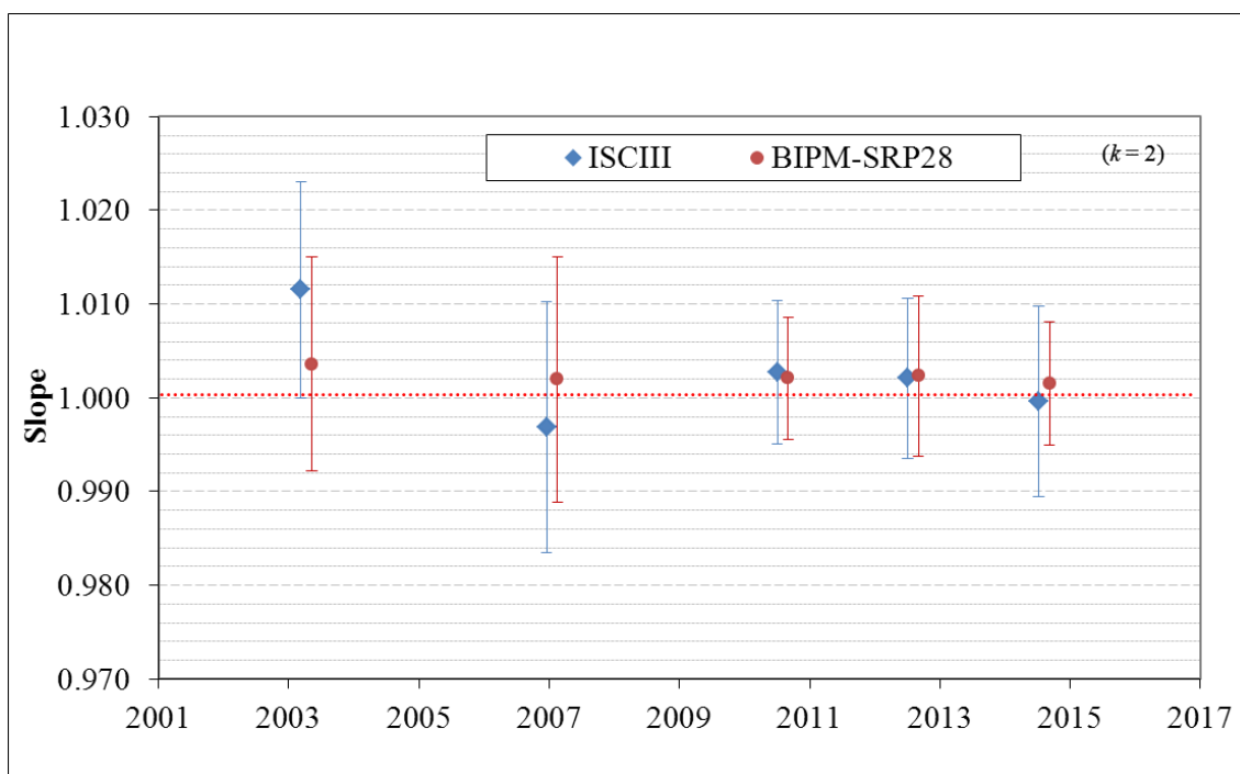
Figure 2 : Results of previous comparisons between SRP27, SRP28 and ISCI-III-SRP22 realised at the BIPM. Uncertainties are calculated at k = 2 , with the uncertainty budget in use at the time of each comparison.
