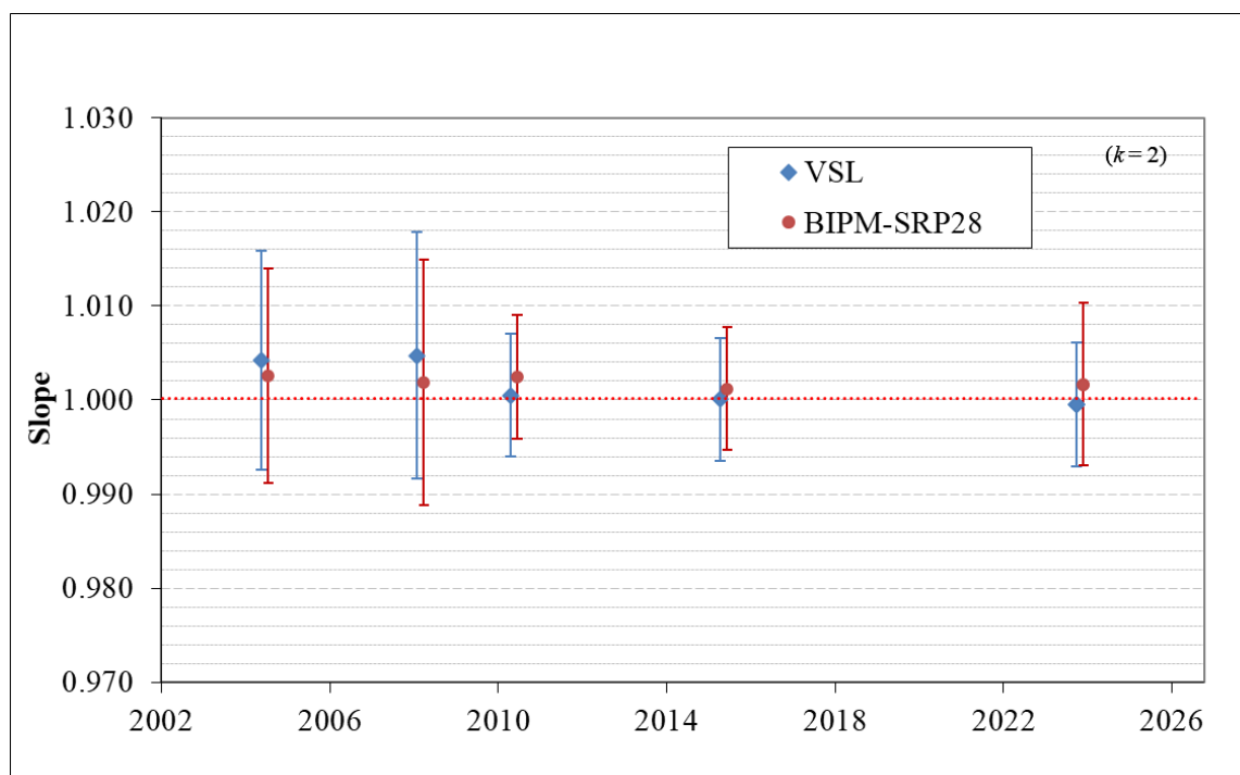
Figure 2: Results of previous comparisons between SRP27, SRP28 and VSL-UMEG26 realised at the BIPM. Uncertainties are calculated at k = 2 , with the uncertainty budget in use at the time of each comparison.
