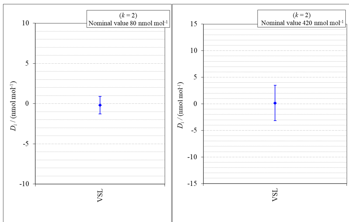
Figure 1: Degrees of equivalence of VSL at the two nominal ozone amount fractions 80 nmol mol -1 and 420 nmol mol -1
