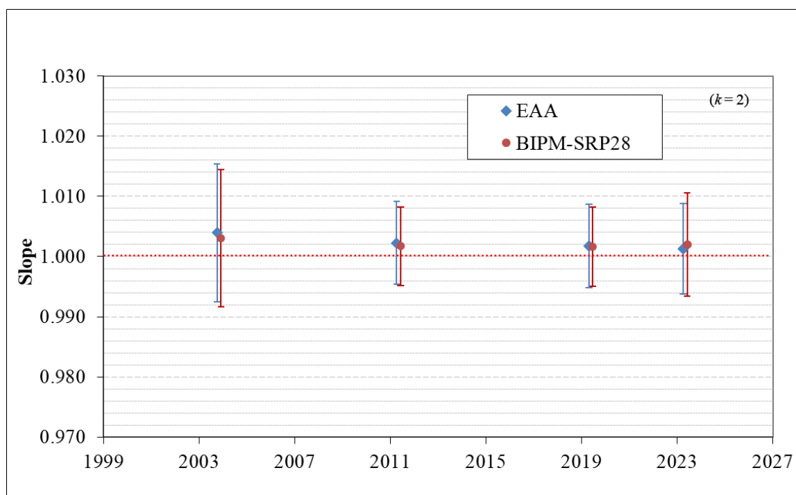
Figure 2: Results of previous comparisons between SRP27, SRP28 and EAA-SRP26 realised at the BIPM. Uncertainties are calculated at k = 2 , with the uncertainty budget in use at the time of each comparison.
