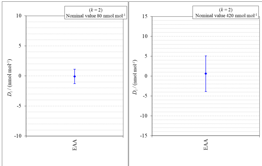
Figure 1: Degrees of equivalence of the EAA at the two nominal ozone amount fractions 80 nmol mol -1 and 420 nmol mol -1
