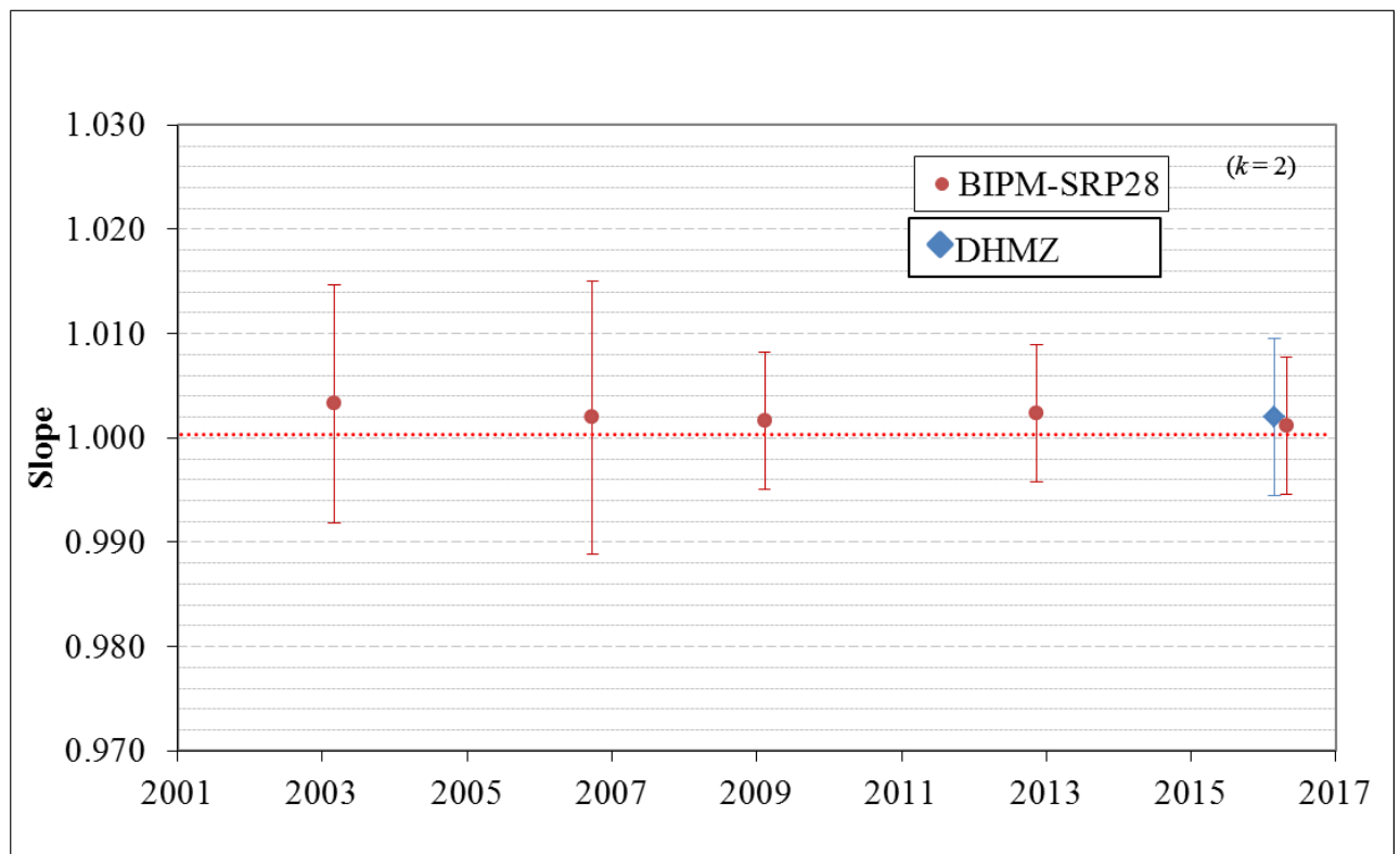
Figure 2 : Results of previous comparisons between SRP27, SRP28 and DHMZ-SRP58 realised at the BIPM. Uncertainties are calculated at k = 2 .
