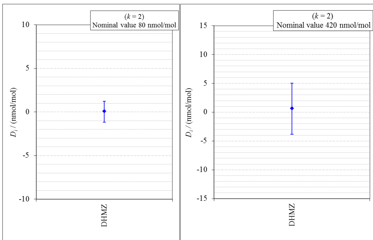
Figure 1: degrees of equivalence of the DHMZ at the two nominal ozone amount-of-substance fractions 80 nmol/mol and 420 nmol/mol
